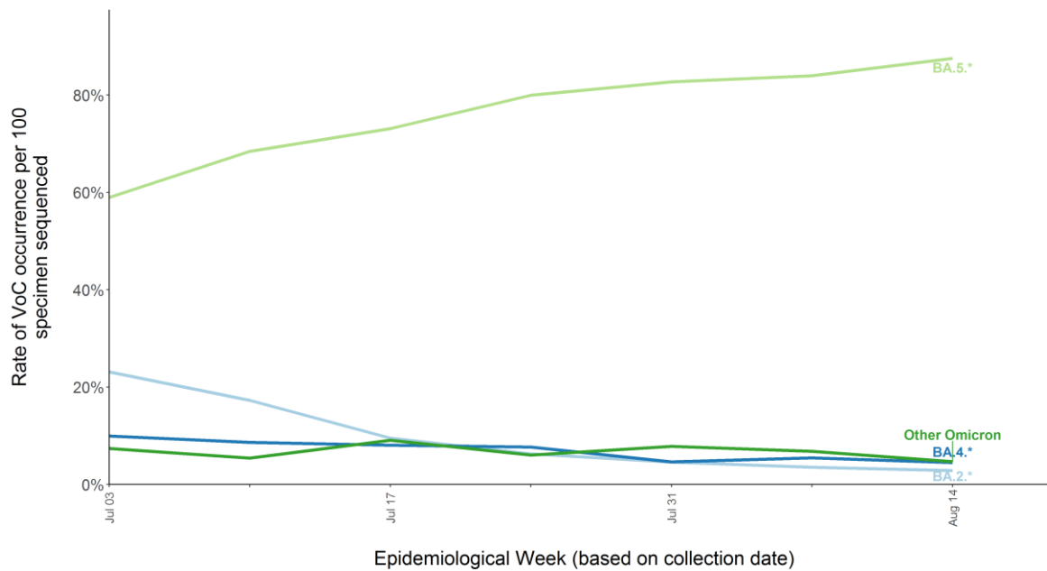
Figure 3. Proportion of lineages # sequenced over the past 6 weeks from 03 July, 2022 to 14 August, 2022
