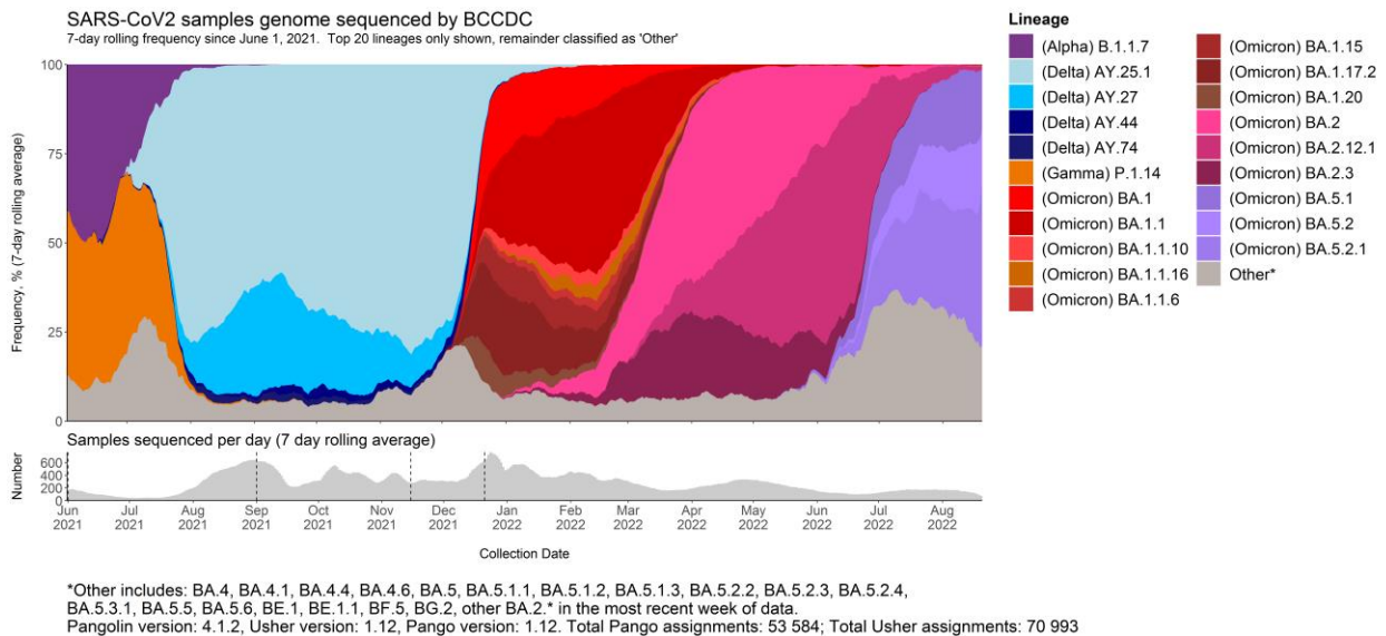
Figure 1. Twenty most prevalent lineages in British Columbia, June 1, 2021 - August 20, 2022**
