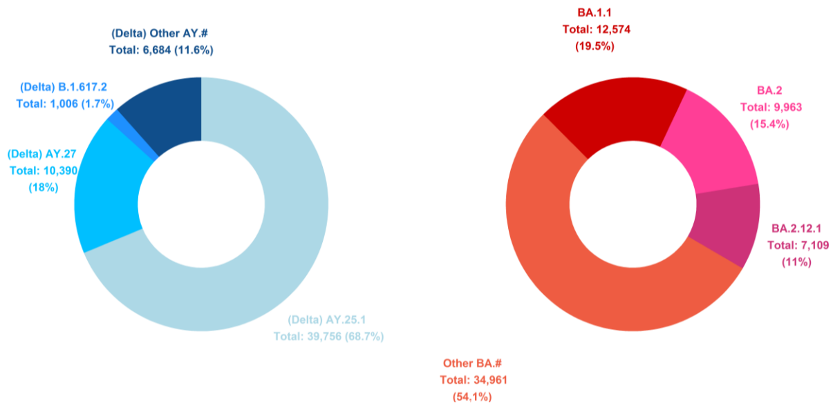
Figure 5. Cumulative Distribution of the three most prevalent Delta and Omicron lineages**
