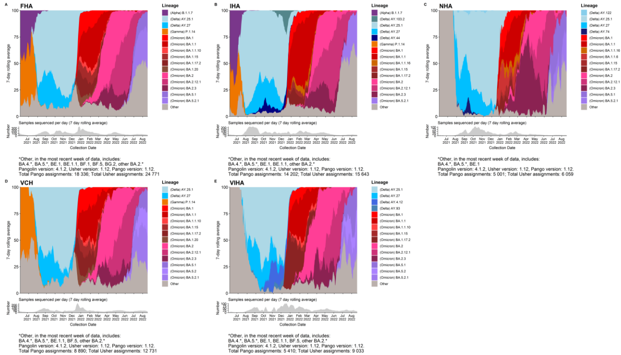
Figure 2. Fifteen most prevalent lineages in British Columbia by Health Authority, between June 1, 2021 - August 20, 2022
